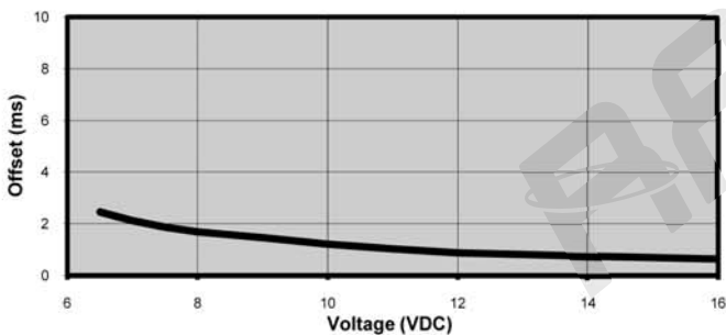
Voltage Sensitivity Summary, 6-16V
