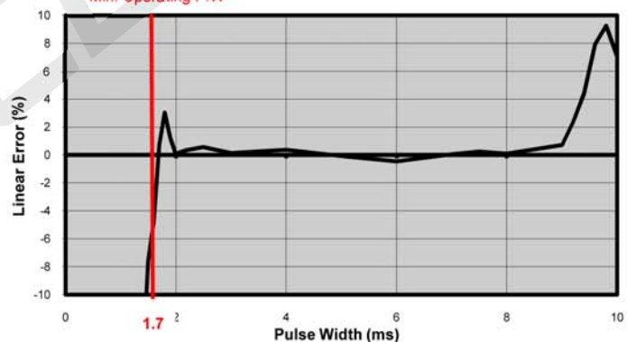
Min. Operating P.W Linearity Error, 0-10ms
